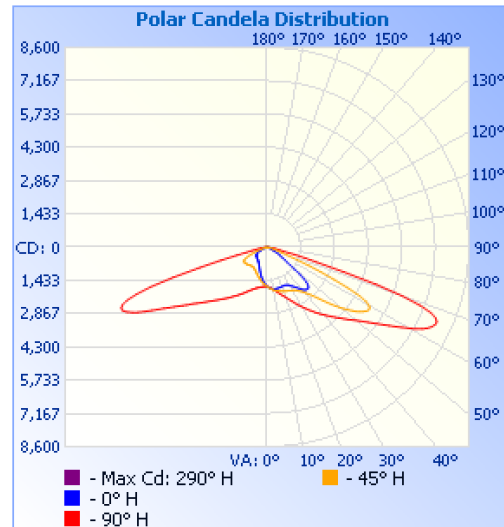
NEPTUNE-100W-30K-T2
