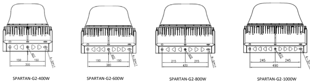
Fig. 1 Measurements of bracket mounting holes
