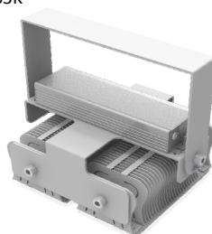
Cross-Bracket Mounting
